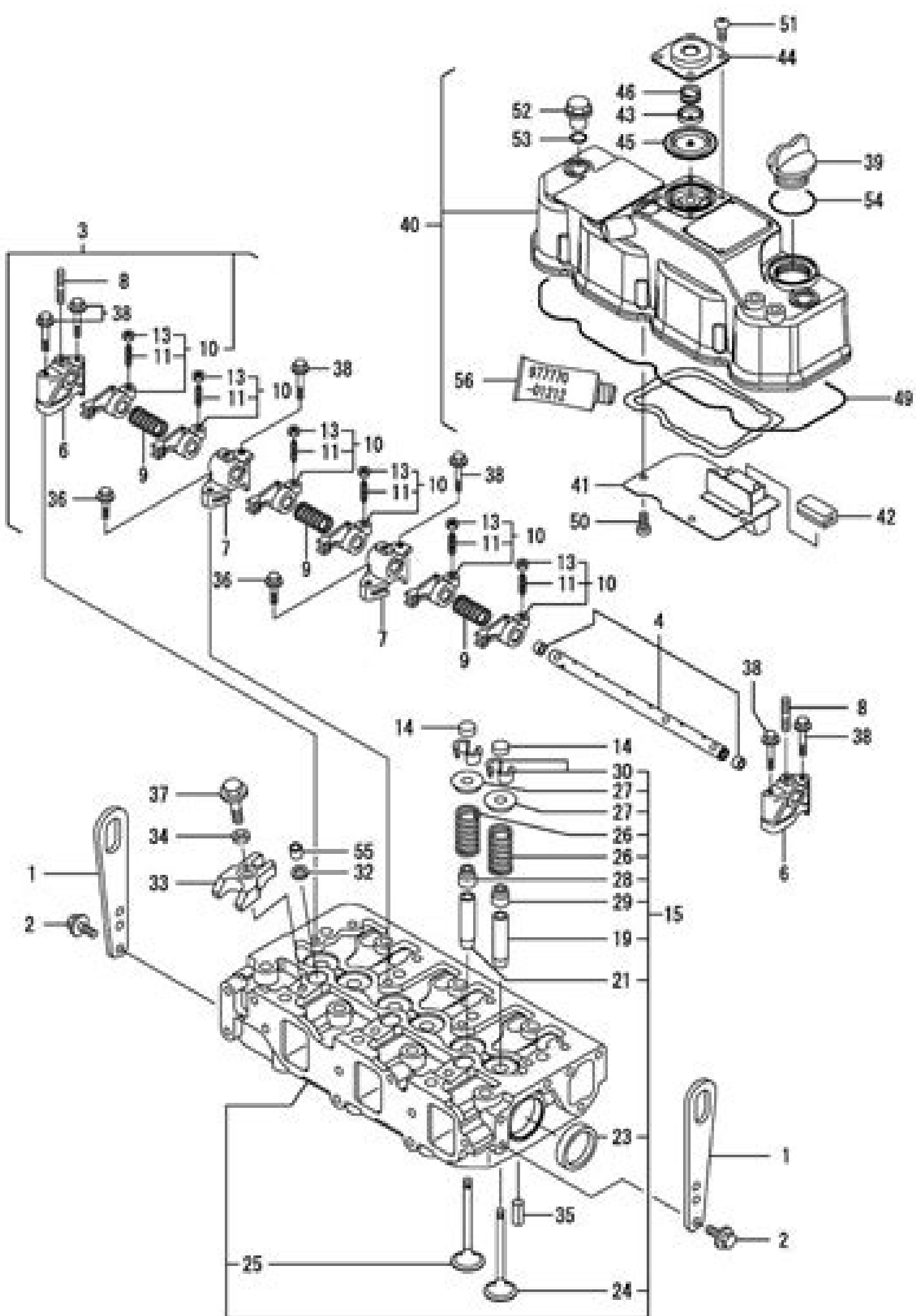
Fig.4. CYLINDER HEAD & BONNET
